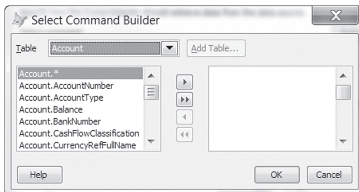
Figure 3. This form from the CursorAdapter Builder uses SQLTables() and SQLColumns() to retrieve data about an ODBC data source.
